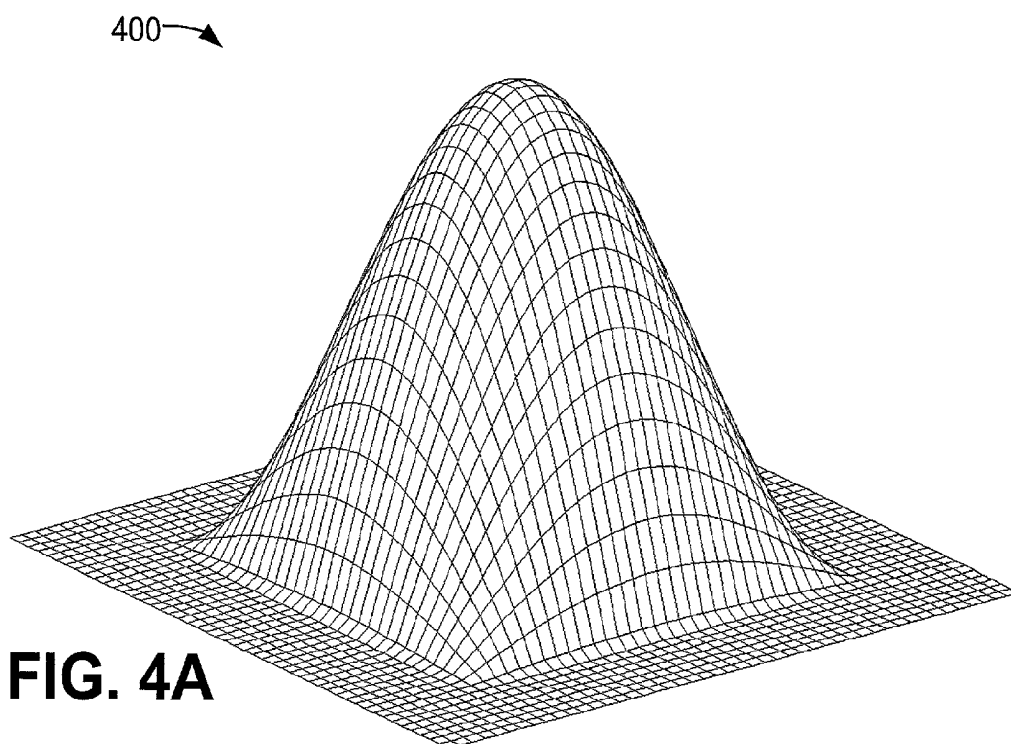
Beam Pattern For Separable Apodization
