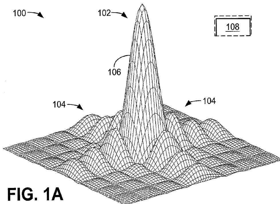
Beam Pattern For Unapodized Aperture
