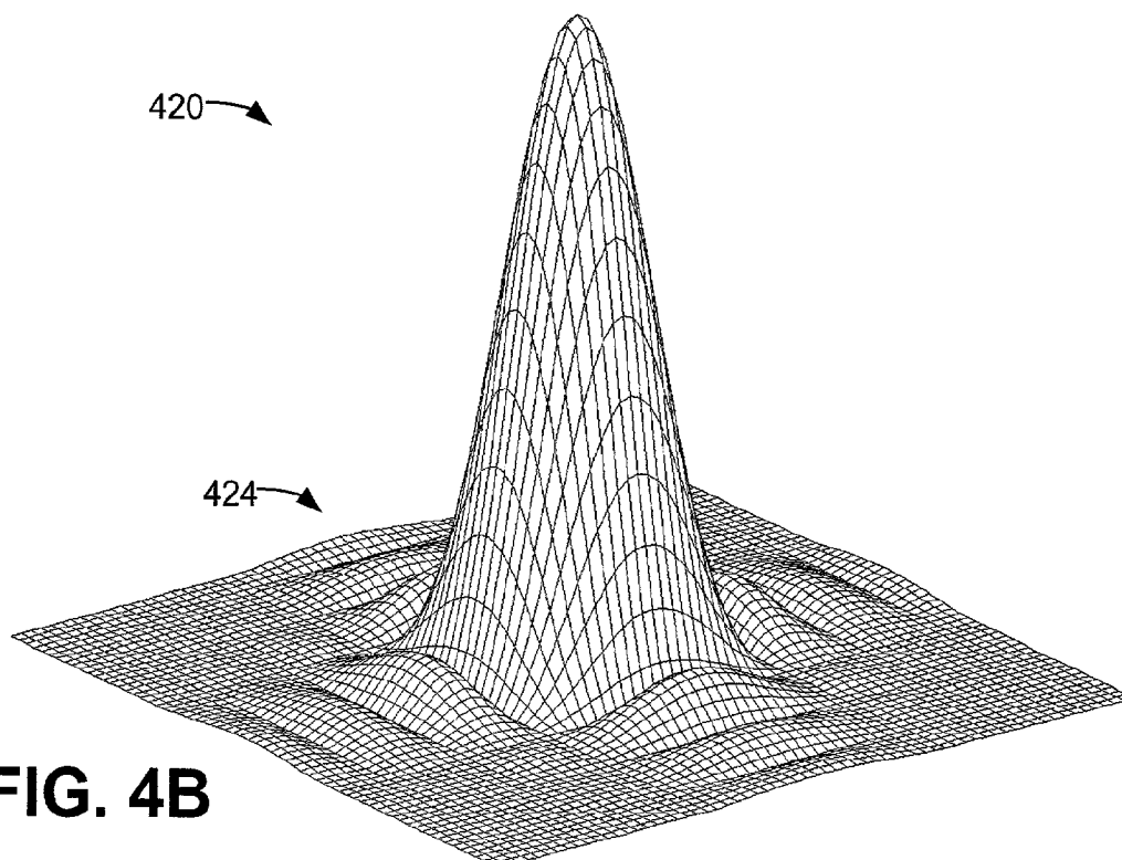
Beam Pattern For Separable Apodization
