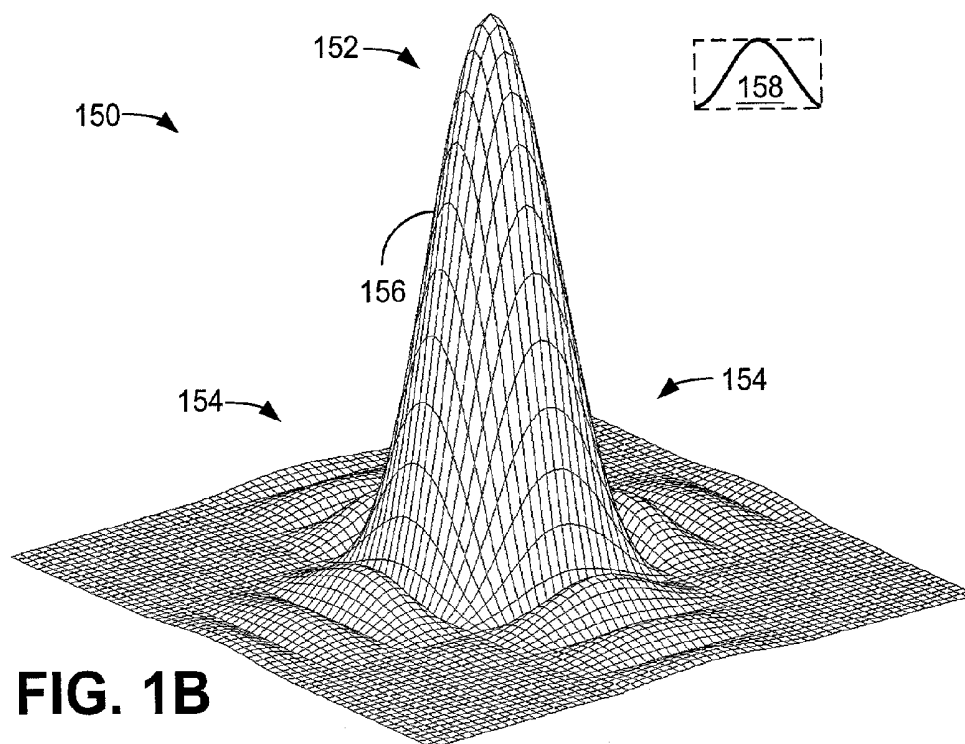
Beam Pattern For Separable Apodization
