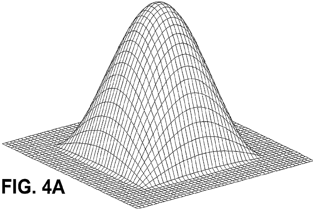
Beam Pattern For Separable Apodization
