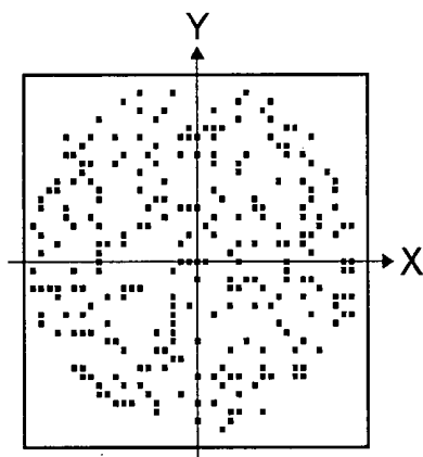
ARRANGEMENT PATTERN OF ELEMENTS FOR RECEPTION
