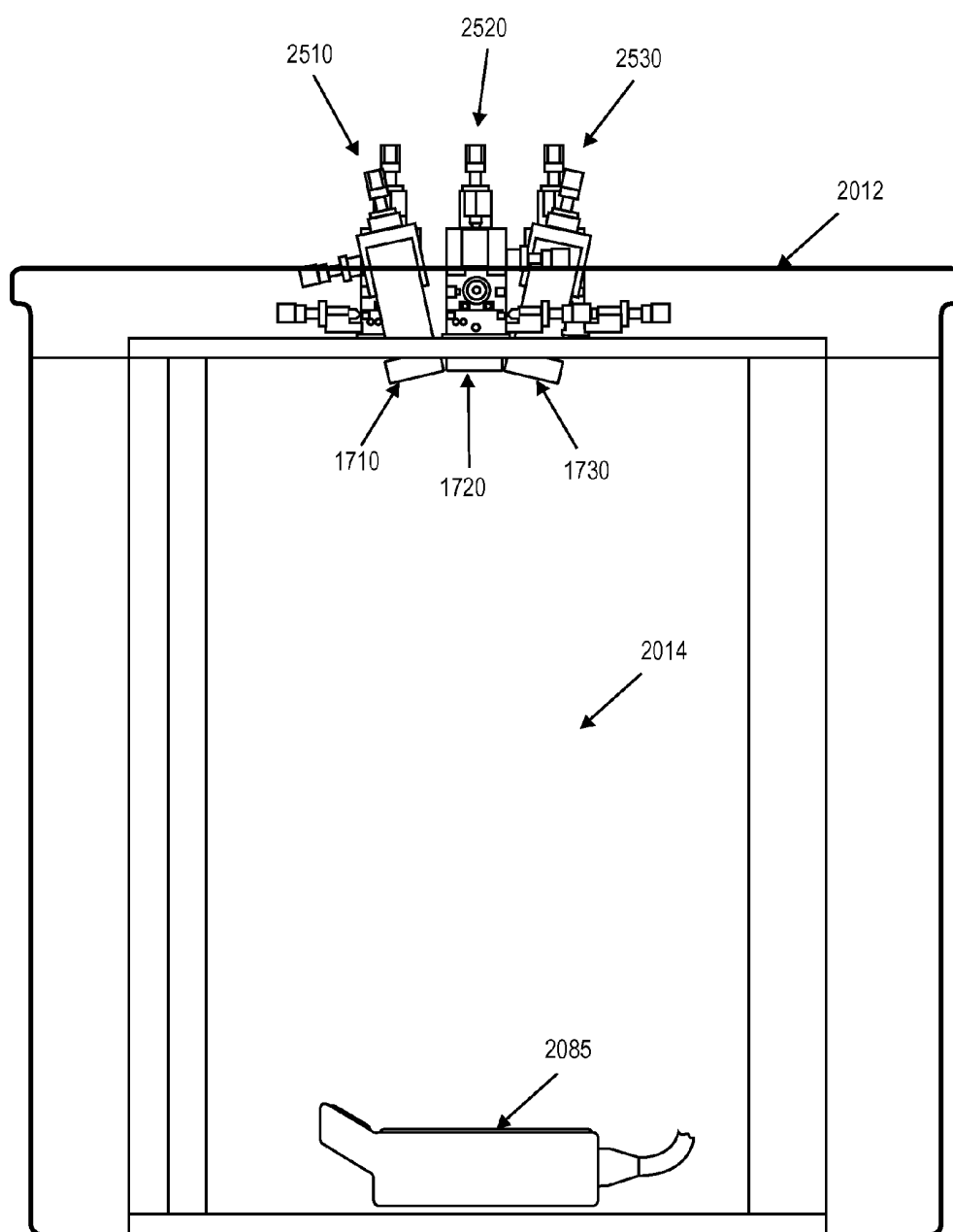
ASSEMBLED TEST FIXTURE IN TANK
