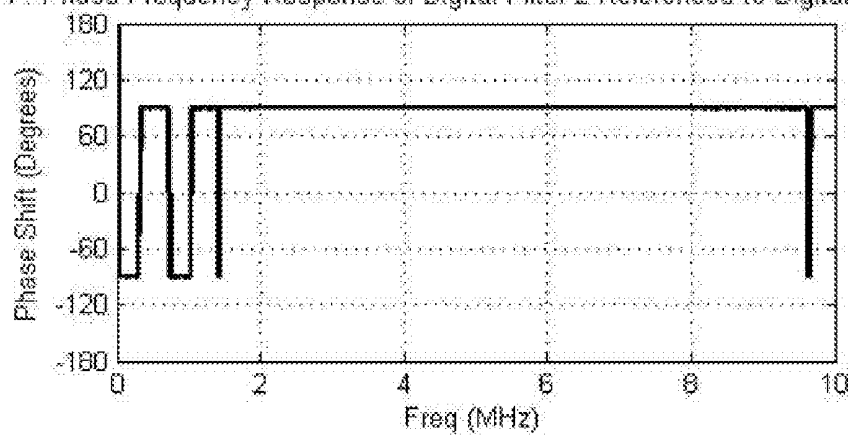
F. Phase Frequency Response of Digital Filter 2 Referenced to Digital Filter 1
