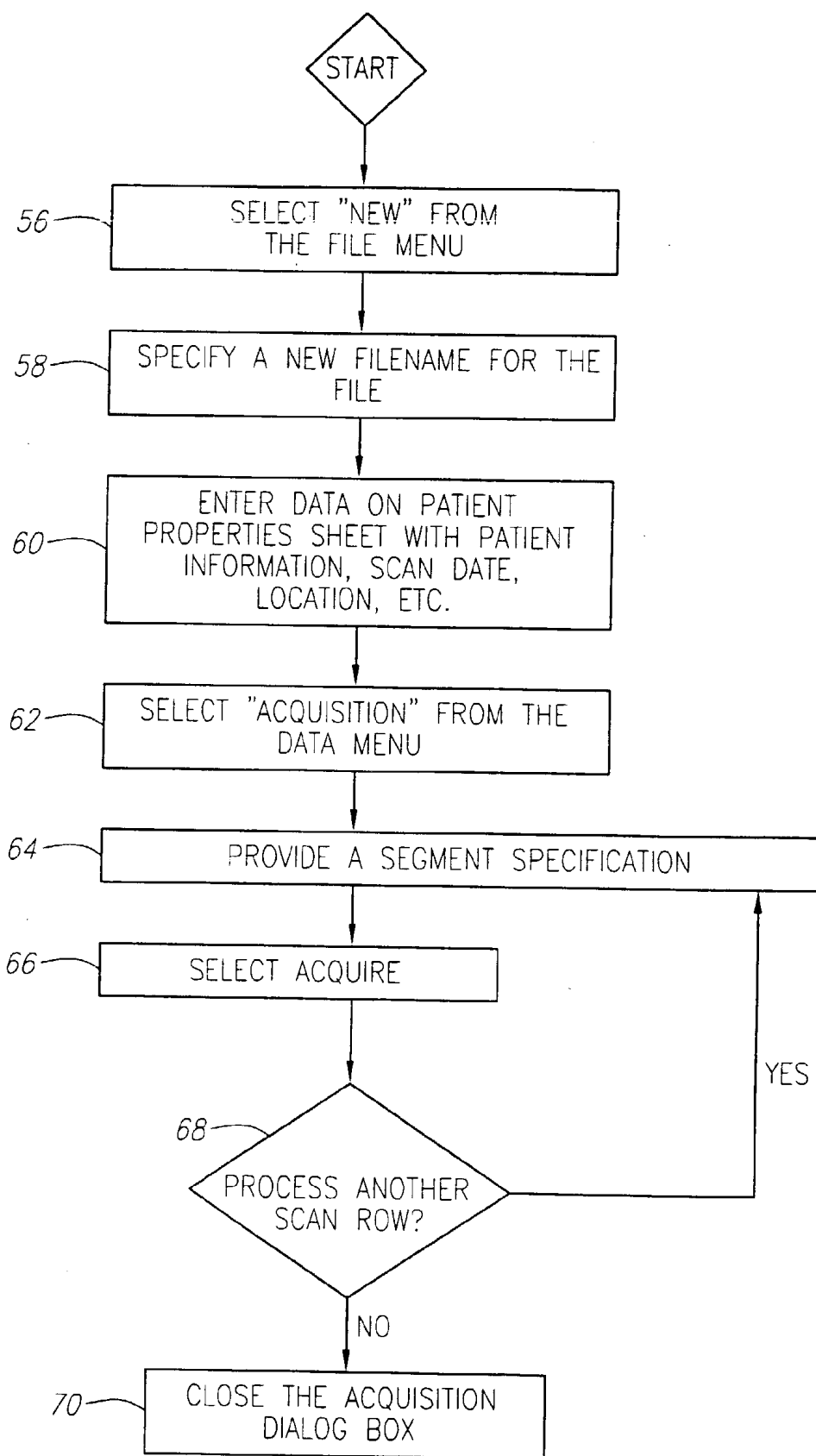
FIG. 7 FILE CREATION USER INTERFACE
