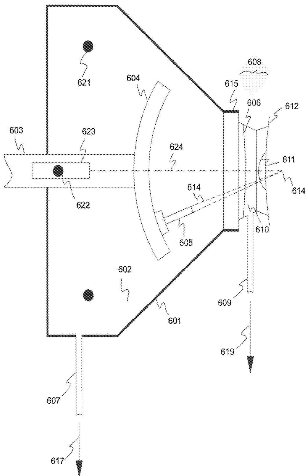
Figure 6 (Prior Art)
