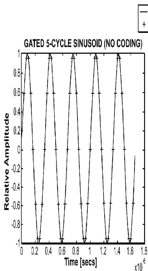
5-CYCLE 3 MHz SINUSOID WITHOUT SPREAD-SPECTRUM CODING
