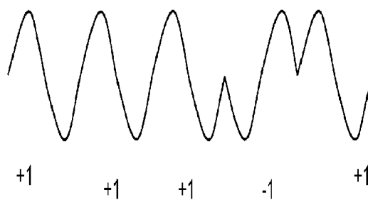
FIG. 24B Base Pulse convolves with 5-chip Barker code
