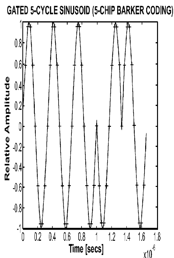
GATED 3 MHz SINUSOID WITH 5-CHIP BARKER CODING [1 1 1 -1 1]
