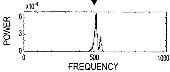
SPECTRUM BEFORE PASSING THROUGH WALL FILTER
