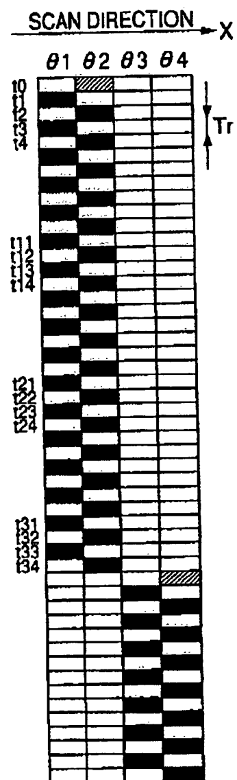
FIG. 10B PRIOR ART
