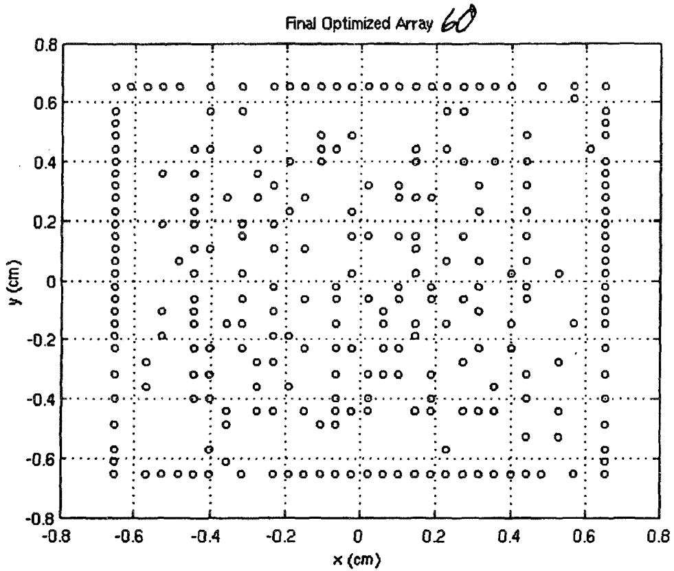
Figure 5: Final element locations for the transmit sparse array. The 256 element locations are confined to the central 32 \times 32 elements of the fully populated array. These elements are independent and do not overlap the receive array elements.
