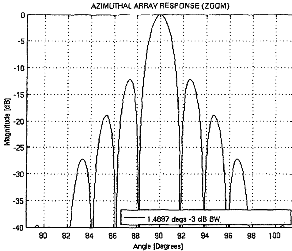
Figure3: Magnifying the azimuthal beam pattern reveals the mainlobe and sidelobe structure. For this case, the beamwidth is approximately 1.5 degrees. The beam pattern is nearly identical to the fully-populated 60x40 element beam pattern.
