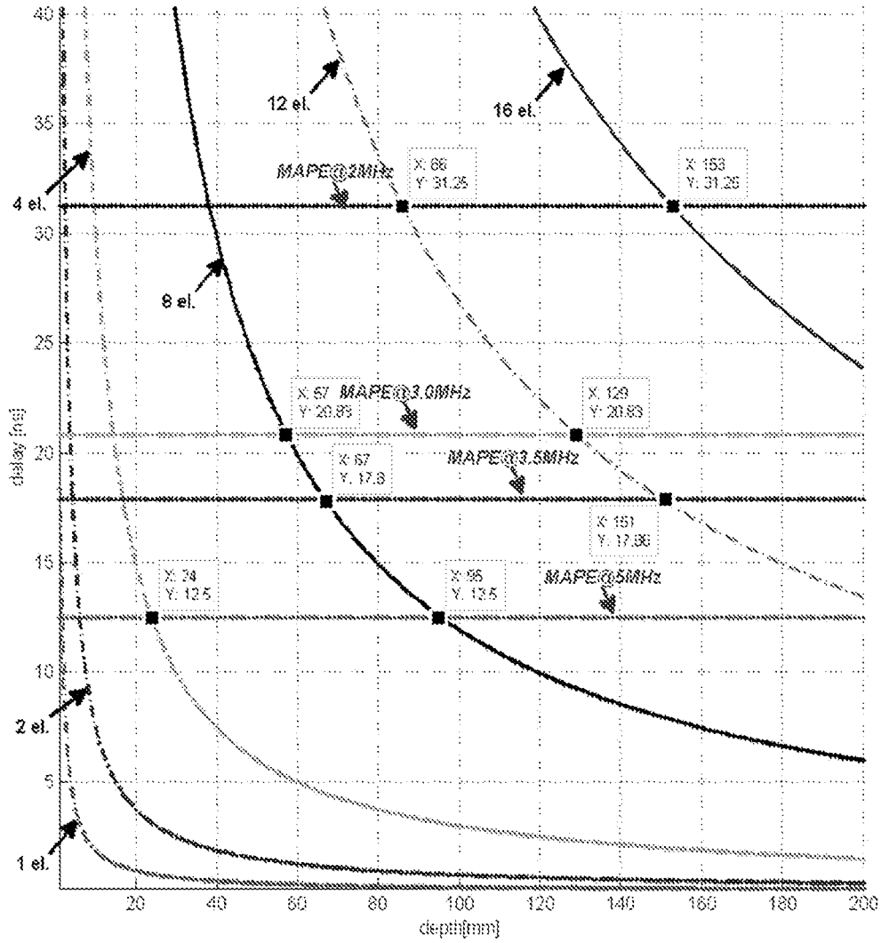
Max. Delay Error at Max. Allowed Phase Error MAPE = \pm (\pi/16) for various aperture sizes (directly summed elements) of C5-2
