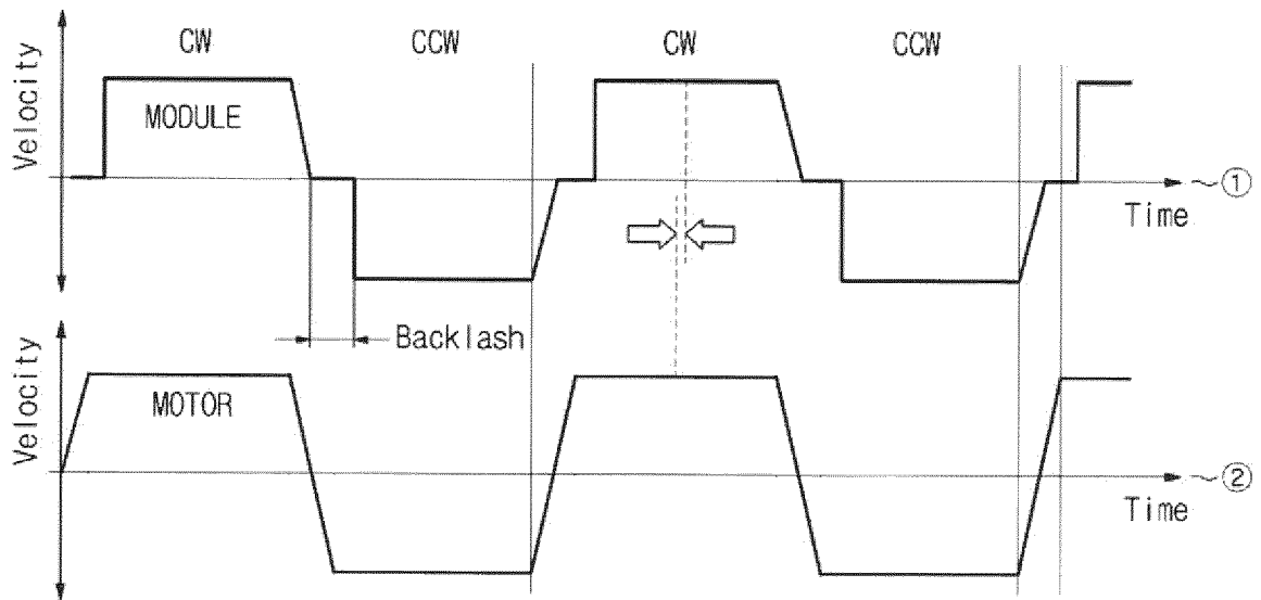
(c) IMAGE BLURRING CAUSED BY BACKLASH
