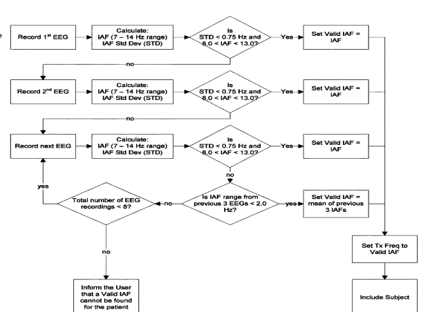
EEG Discrimination Algorithm Flowchart
