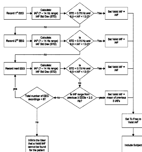
EEG Discrimination Algorithm Flowchart
