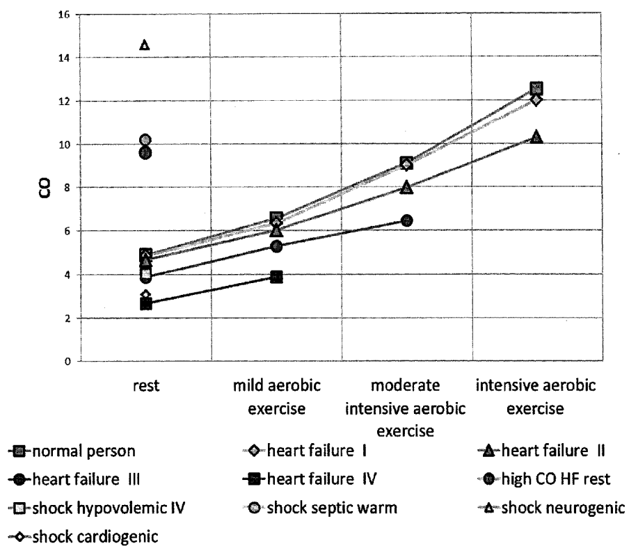
Cardiac Output by morbidity severity and exercise intensity by morbidity severity and exercise intensity (putting the representative/average values (SV, SVR, RR) for each condition)
