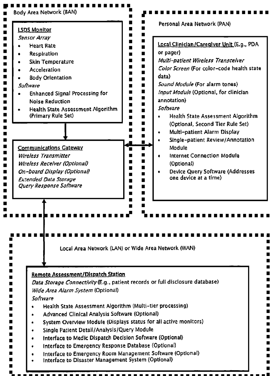
Figure 48 - Block Diagram :Life Signs Detection System
