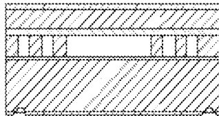
(D) Oxidize separate Si wafer, bond wafers, then grind/polish top layer to 20 \mu m, LPCVD oxide
