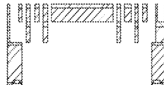
(H) Use backside align marks to create DRIE scanner release window
