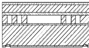
(D) Oxidize separate Si wafer, bond wafers, then grind/polish top layer to 20µm, LPCVD oxide
