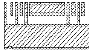
(G) RIE insulation oxide, DRIE etch to trim stator features to match rotors & create bond pad vias
