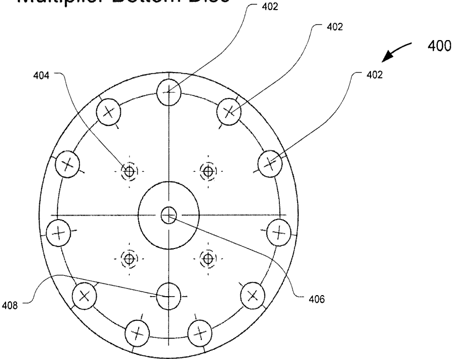
Multiplier Bottom Disc
