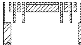
(H) Use backside align marks to create DRIE scanner release window
