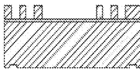
(C) BOE oxide, DRIE coarse stator features in silicon device layer
