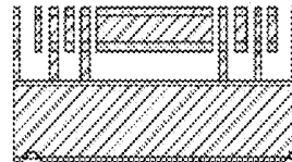
(G) RIE insulation oxide, DRIE etch to trim stator features to match rotors & create bond pad vias
