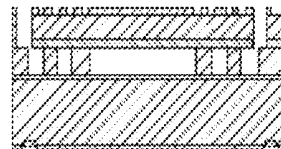
(E) DRIE expose front align marks, RIE oxide with bond pads & exact microscanner features
