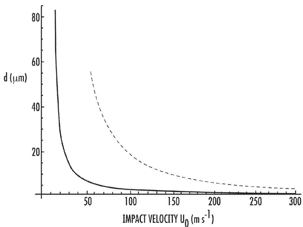
CRITICAL DIAMETER FOR SPLASHING TO OCCUR ON BAFFLE
