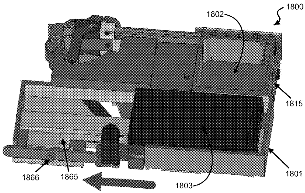
Initial position of the lancet cartridge 1803
