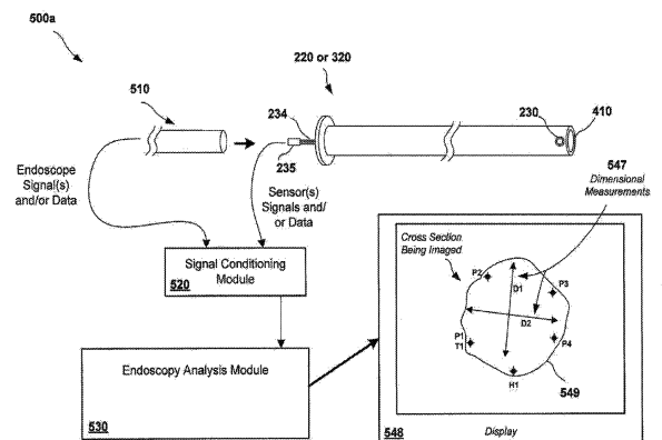
Example Sensor Enhanced Endoscopy System
