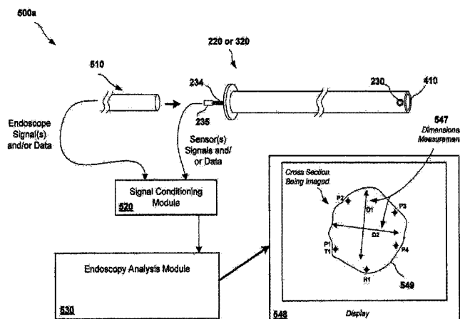
Example Sensor Enhanced Endoscopy System
