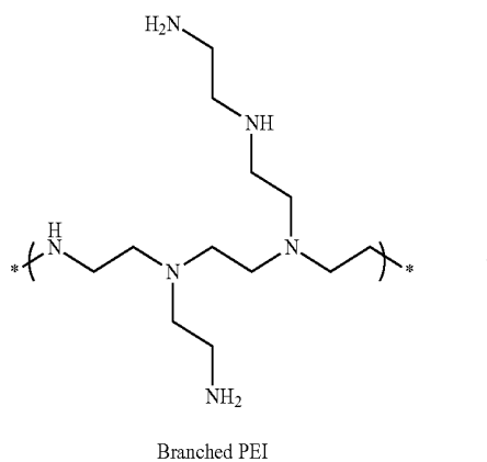
Scheme 5:
