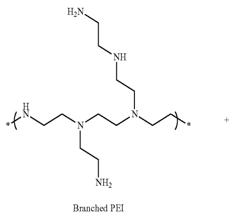
Scheme 3:
