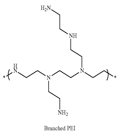
Scheme 6:
