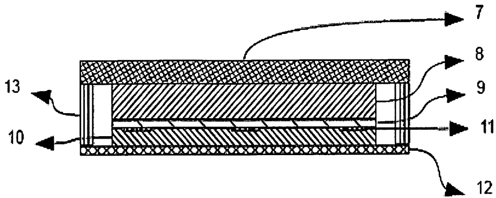
Fig. 3A Cross sectional view of applicator
