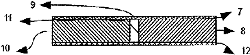
Fig. 7A Cross sectional view of applicator
