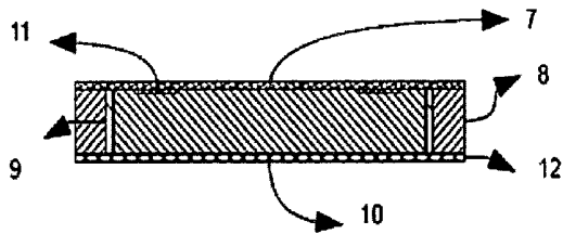
Fig. 4A Cross sectional view of applicator
