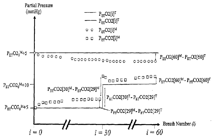
Figure 6 Tuning
