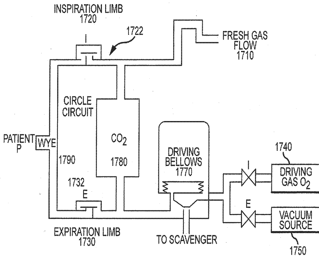
ANESTHESIA MACHINE WITH ACTIVE EXHALATION
