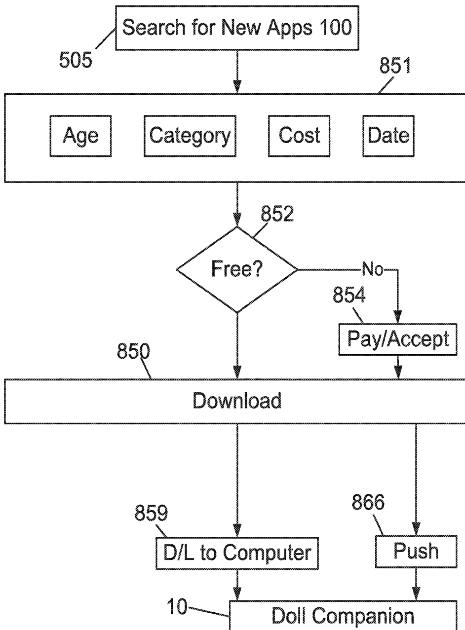
FIG. 16 Application Administrative Interface
