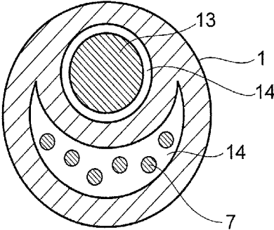
FIG.1 (Related Art)
