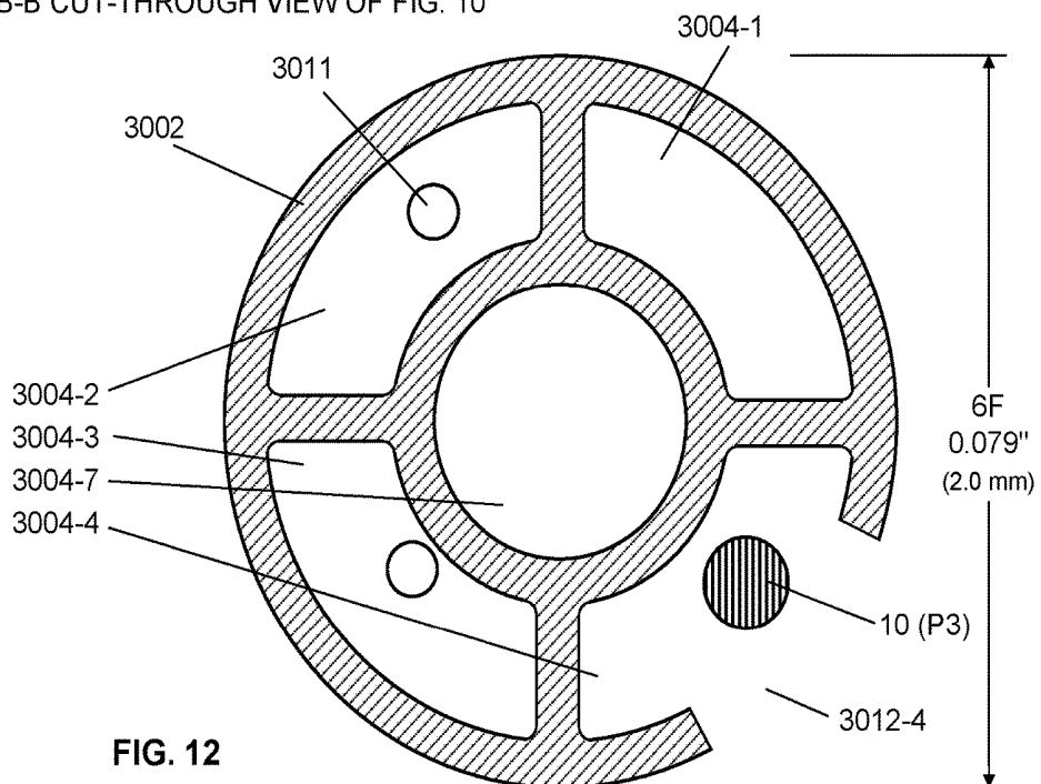
B-B CUT-THROUGH VIEW OF FIG. 10
