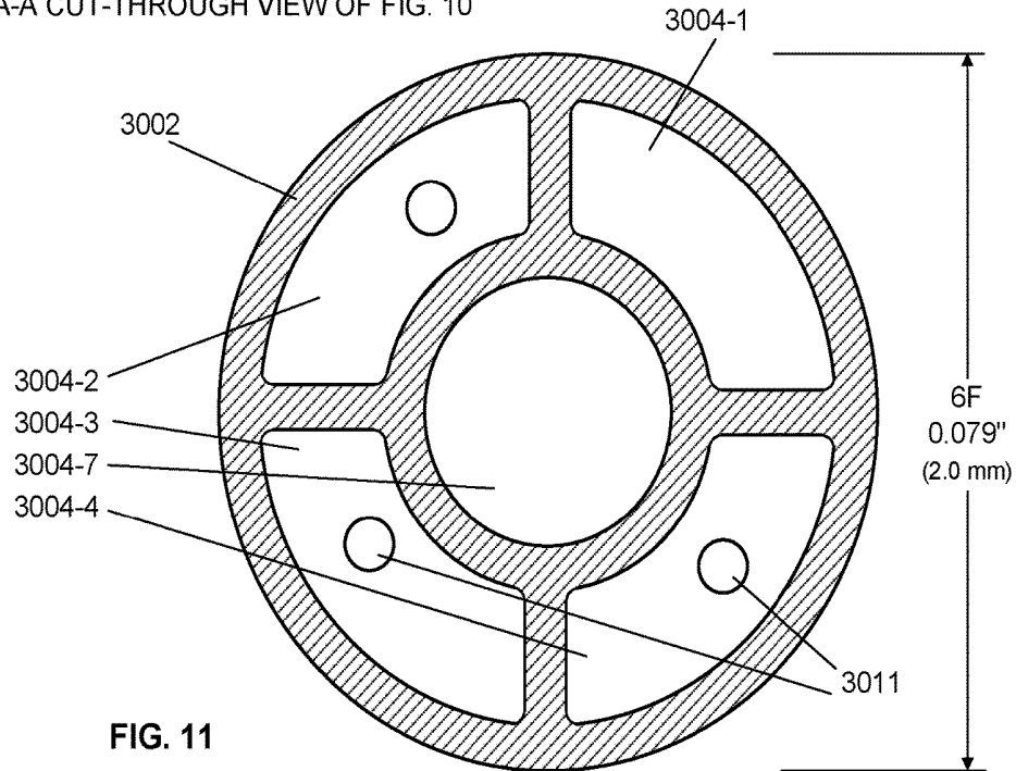
A-A CUT-THROUGH VIEW OF FIG. 10
