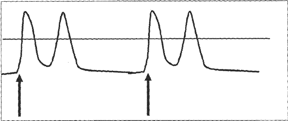
Figure 4: The acoustic envelope.
