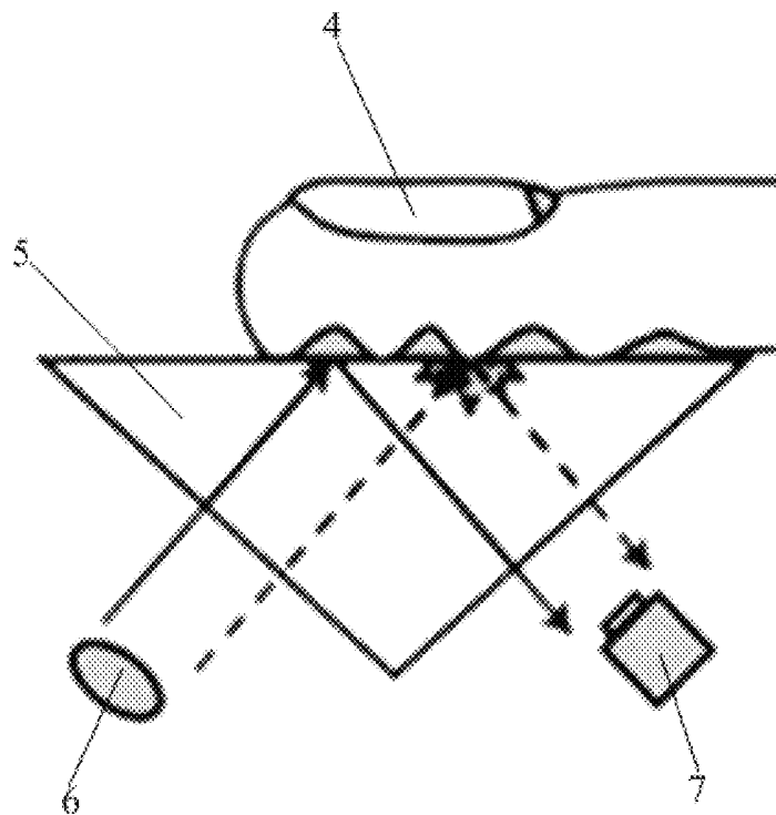
Fig. 1 (Prior Art)
