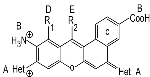
Scheme 3. Structure of Generic pH Sensitive Dye for Specific Action as a Lactate/H + SMMR
