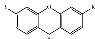
Basic Xanthene Structure
