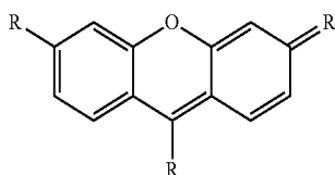
Generic Fluorophore Structure I for SubMol candidate
