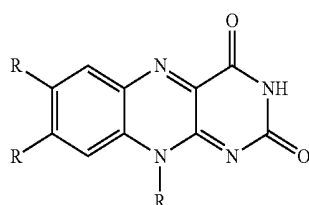
Structure of FAD FL SubMol Moiety
