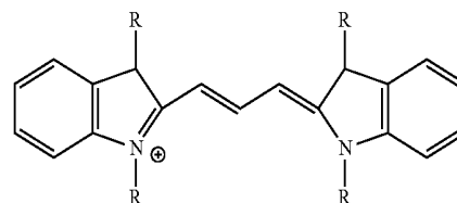
Cyanine dye structure
