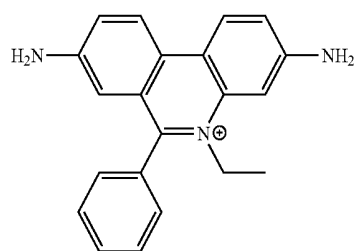
Ethidium Bromide, shown without the counter ion.
