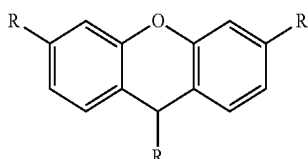
Structure of Basic Xanthene Molecule useful as a core SubMol structure
