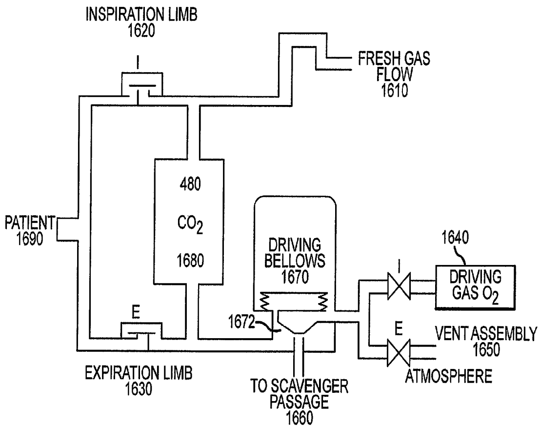
ANESTHESIA MACHINE
