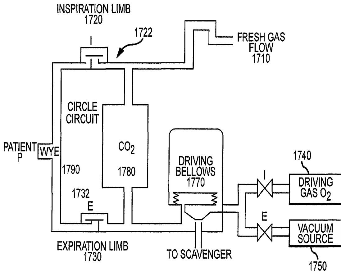
ANESTHESIA MACHINE WITH ACTIVE EXHALATION
