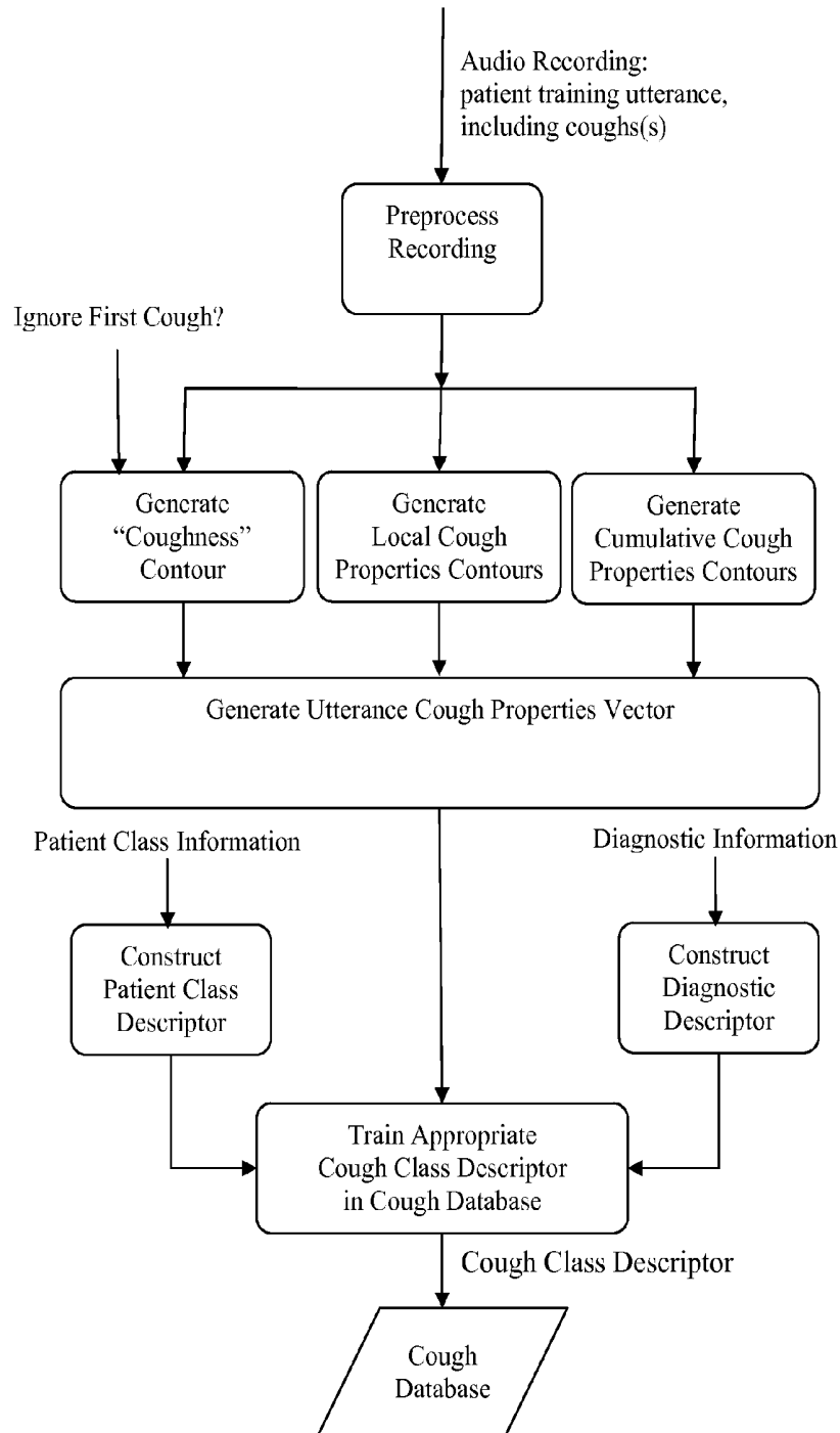
FIG. 5: Cough Classifier Top-level Flowchart: Training Mode
