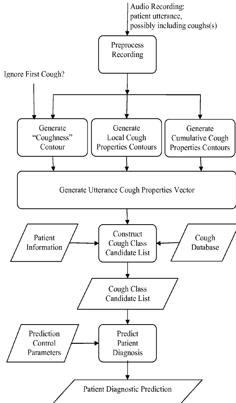
FIG. 3: Cough Classifier Top-level Flowchart: Classification Mode
