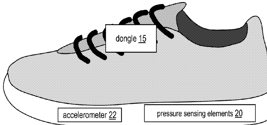
side view
