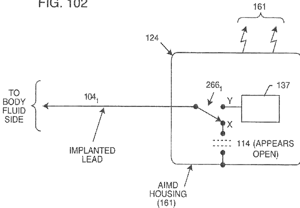
MRI GRADIENT (LOW) FREQUENCY MODEL
