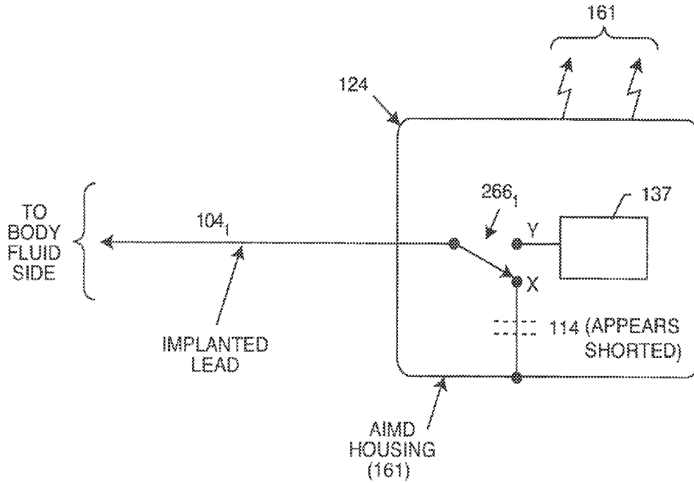
MRI PULSED RF (HIGH) FREQUENCY MODEL
