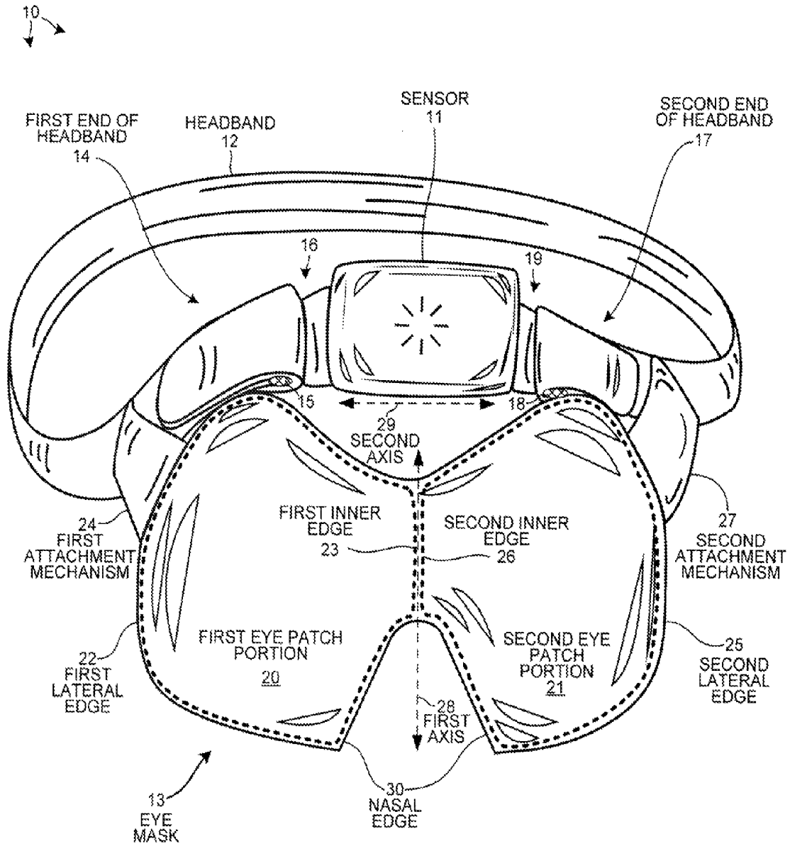
FRONT VIEW (FIRST EMBODIMENT)
