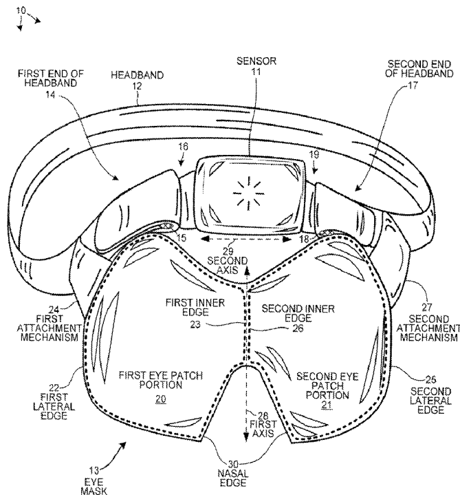
FRONT VIEW (FIRST EMBODIMENT)
