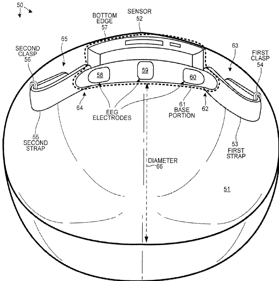
BOTTOM VIEW (SECOND EMBODIMENT)
