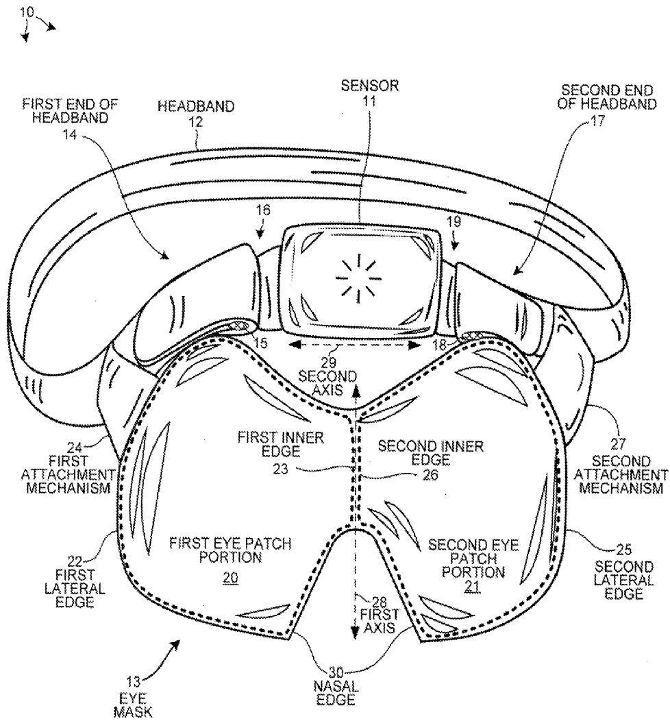
FRONT VIEW (FIRST EMBODIMENT)
