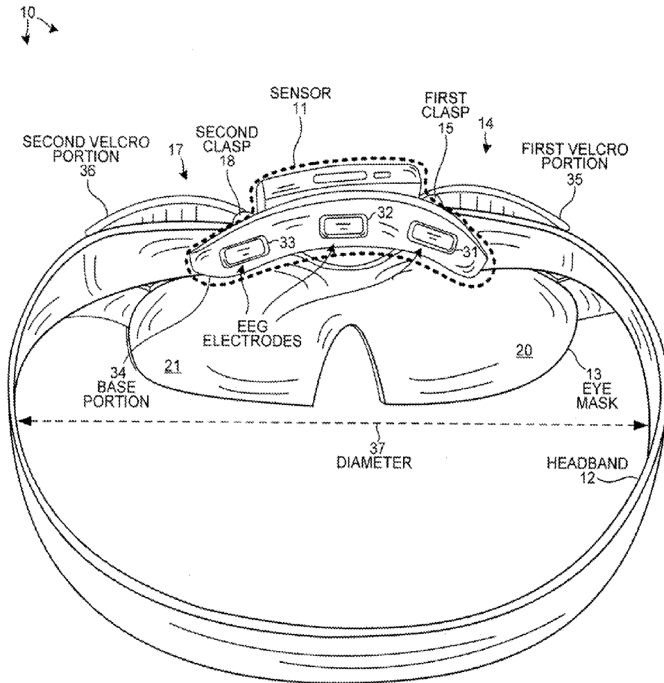
BACK VIEW FIG. 5
