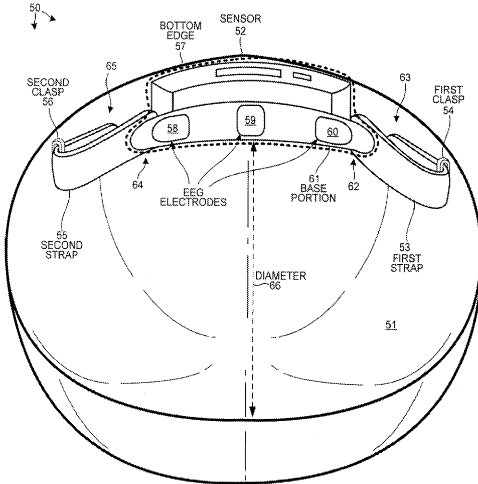
BOTTOM VIEW (SECOND EMBODIMENT)
