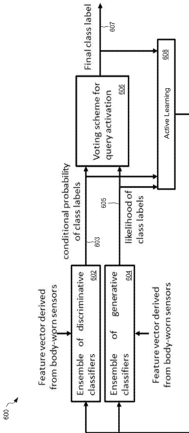
FIG. 6 DIAGRAM OF HYBRID GENERATIVE-DISCRIMINATIVE CLASSIFIER WITH ACTIVE LEARNING
