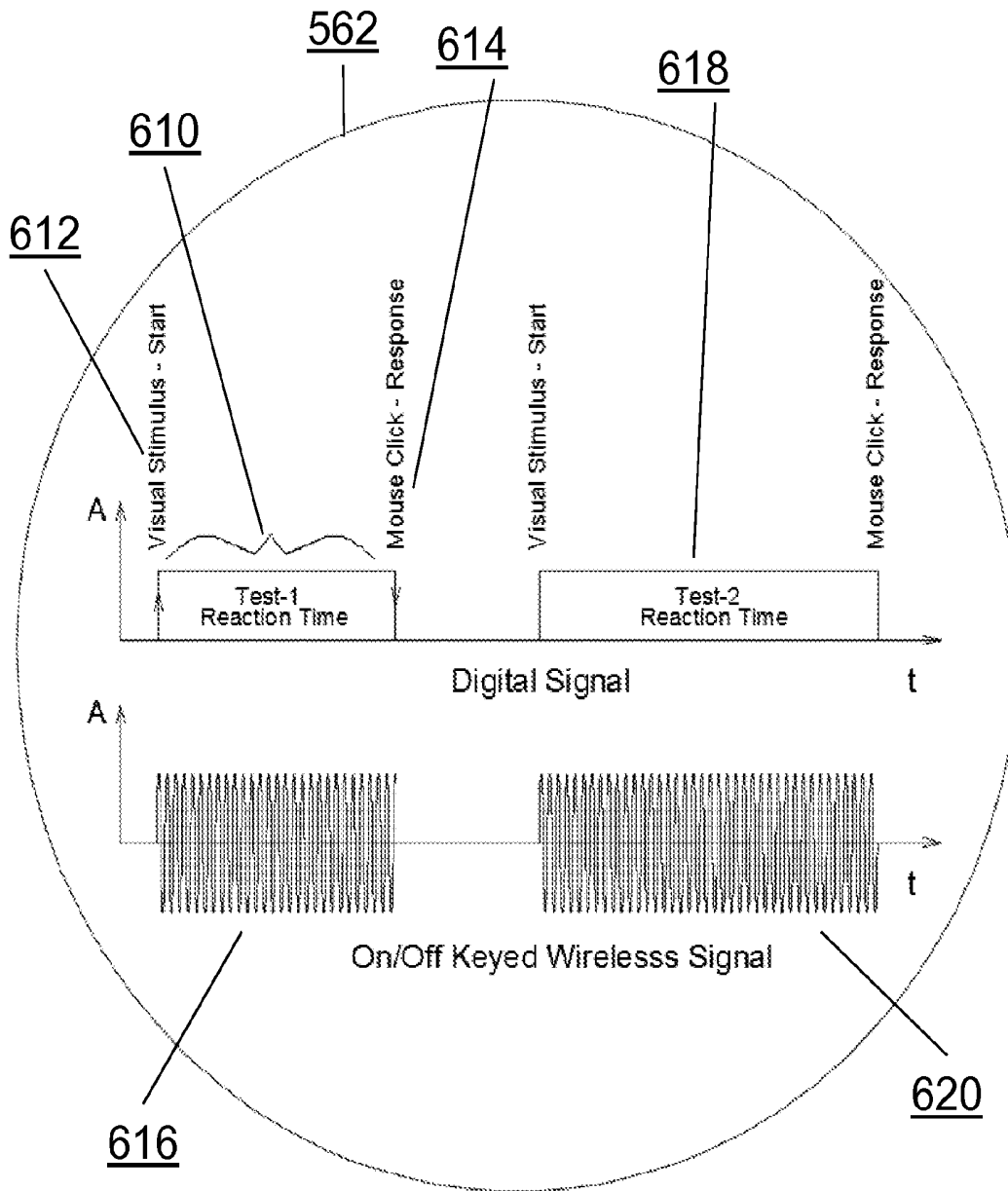
Digital and wireless carrier signals used to send reaction time to EEG Headset
