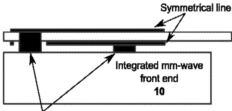
Micro-vias connecting differential mm-wave pins with symmetrical line using polymer engineering
