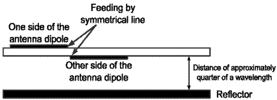
Dipoles, arrangement and reflector
