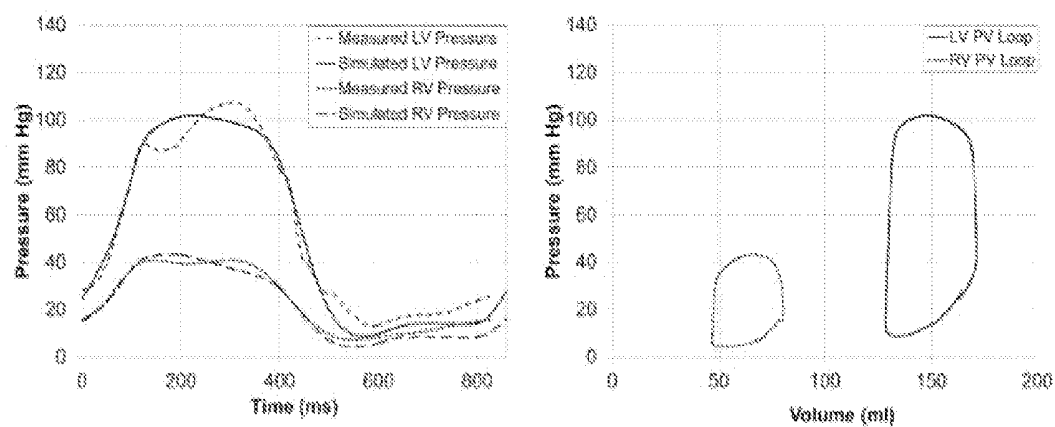
Figure 8: Simulated and Measured LV and RV Pressure and PV Loops.
