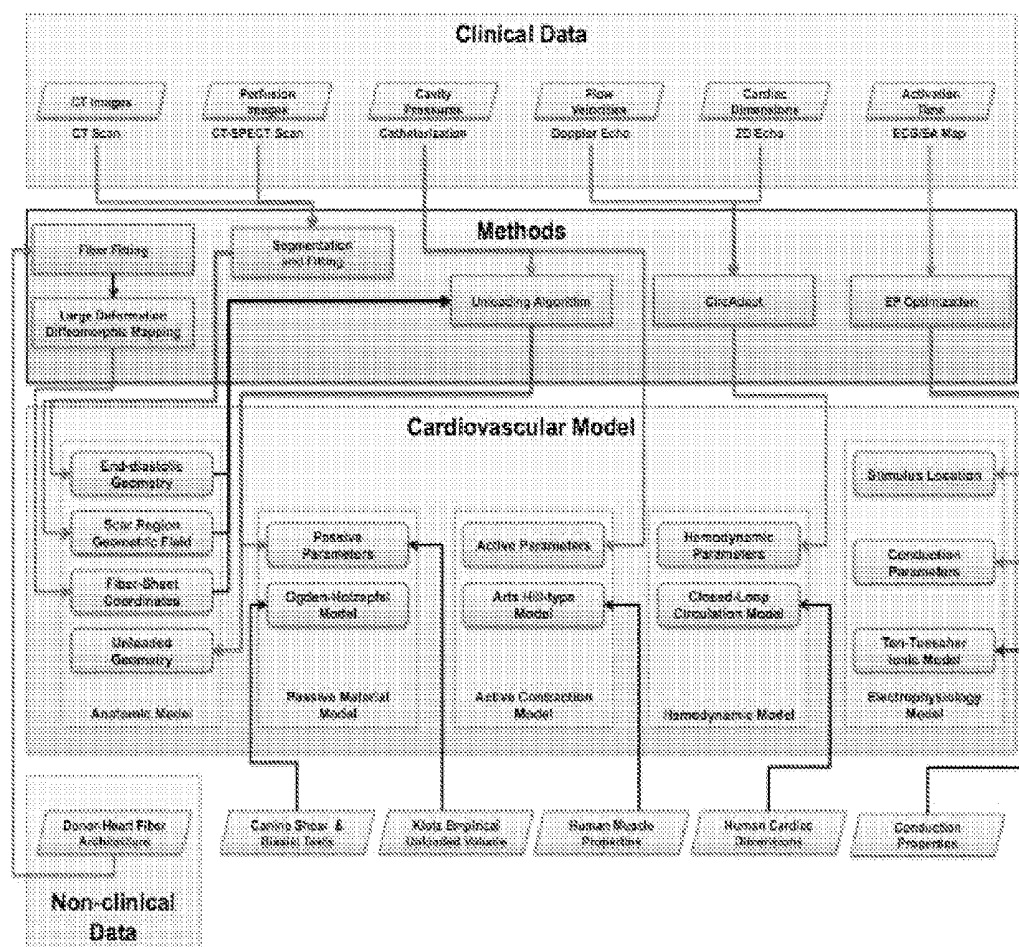
Figure 3: Different components of the patient-specific electromechanics model utilized in its construction.
