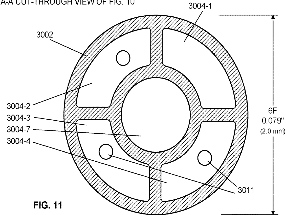
A-A CUT-THROUGH VIEW OF FIG. 10
