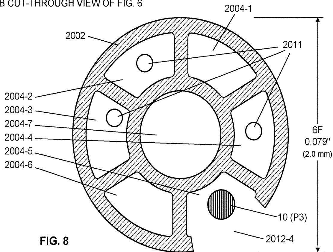
B-B CUT-THROUGH VIEW OF FIG. 6
