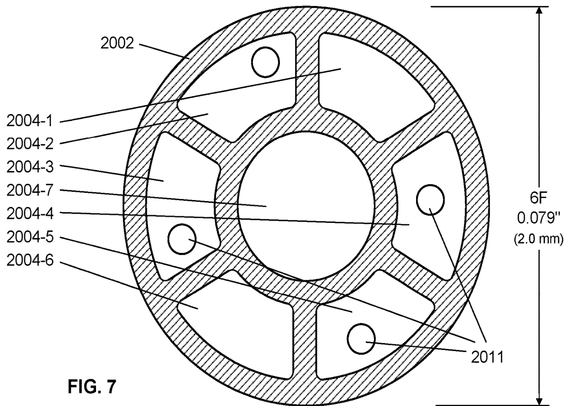
A-A CUT-THROUGH VIEW OF FIGS. 5, 6 AND 9
