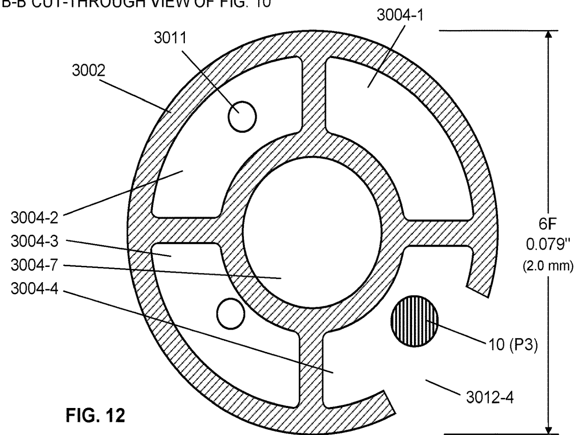
B-B CUT-THROUGH VIEW OF FIG. 10
