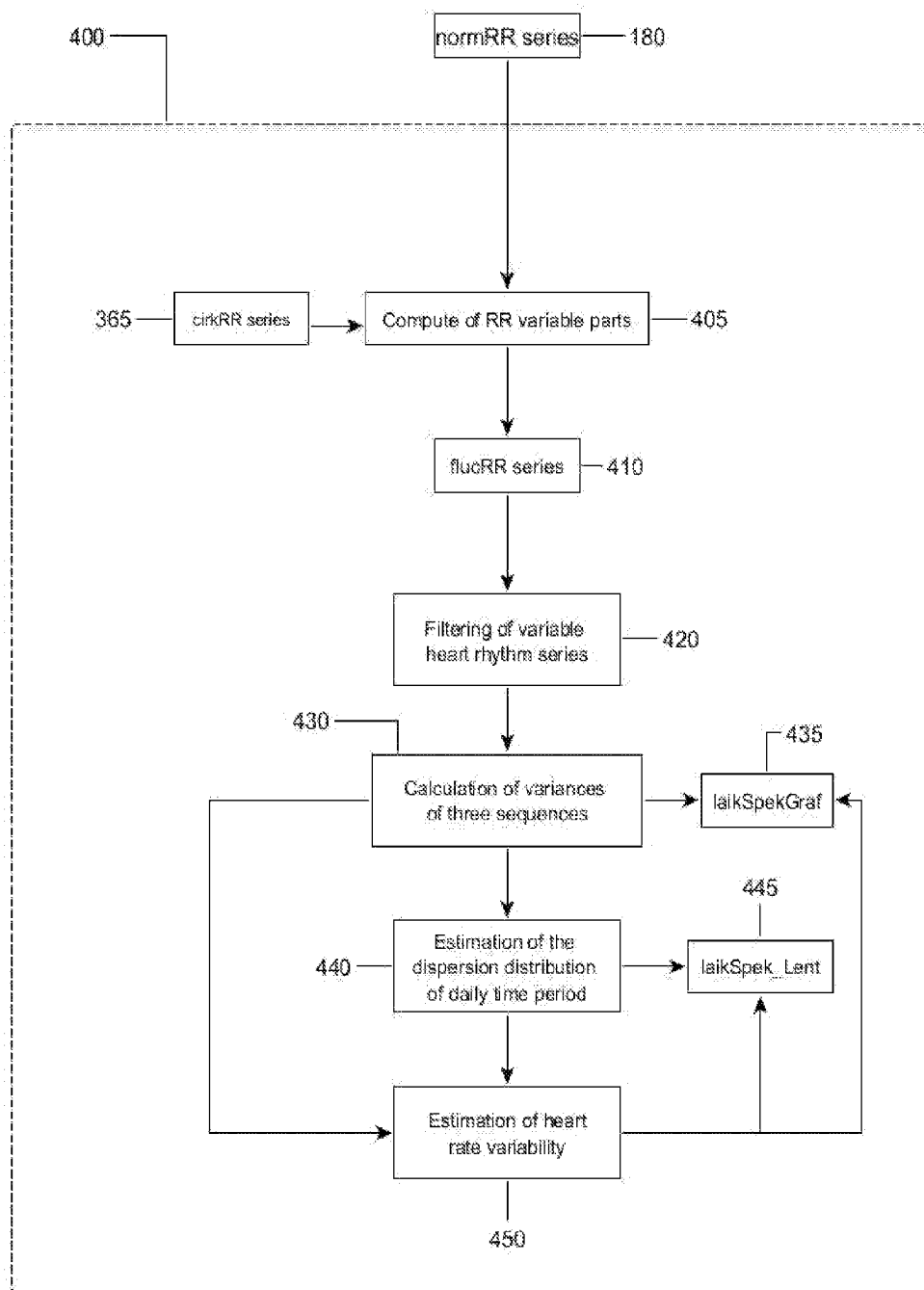
Fig. 5. Block for the analysis of the SNS and PNS regulation criteria of the heart rhythm variable part
