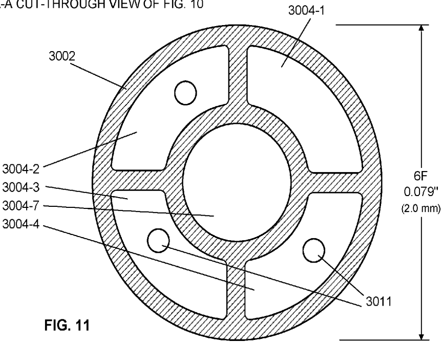
A-A CUT-THROUGH VIEW OF FIG. 10
