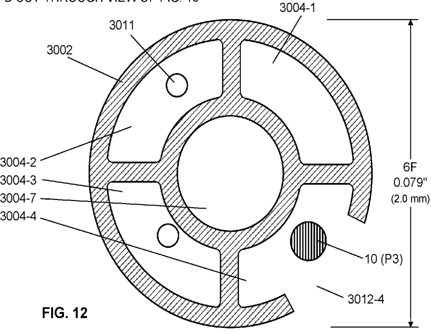
B-B CUT-THROUGH VIEW OF FIG. 10
