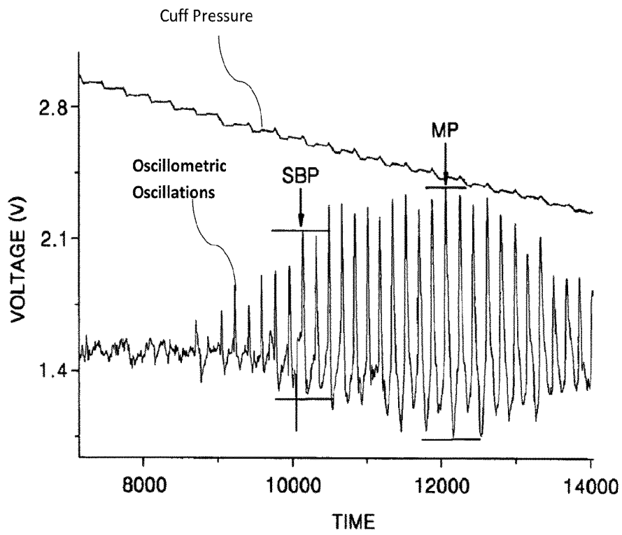
FIGURE 2 (PRIOR ART)
