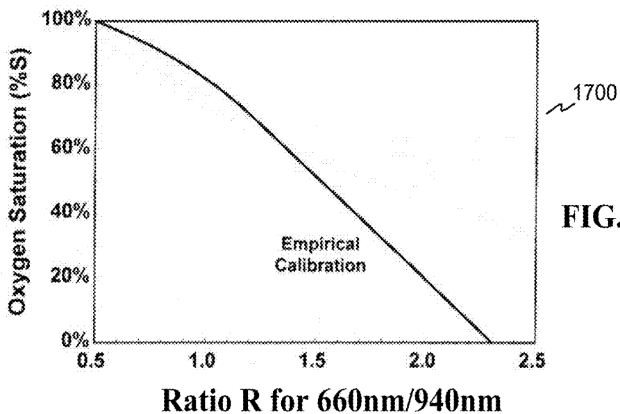
Calibration Curve (R Values) for \text{SpO}_2
