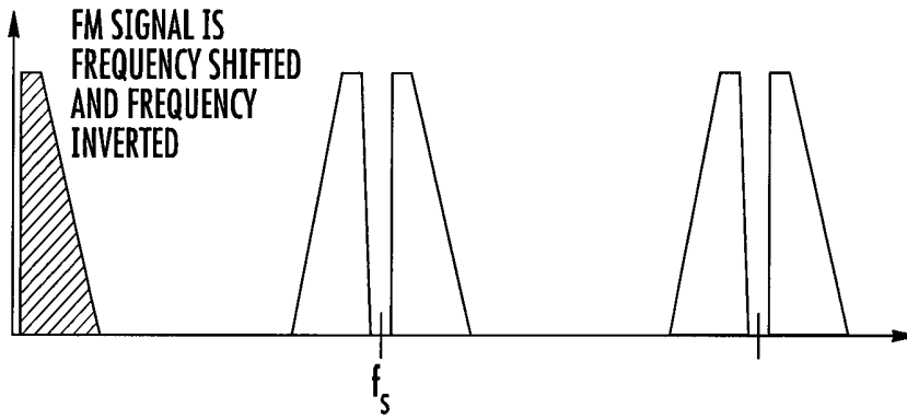
FREQUENCY SPECTRUM AFTER UNDERSAMPLING AT HALF THE ORIGINAL SAMPLING RATE
