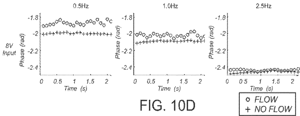
Elongate Member #1 Resistive Member #4: Phase Plot
