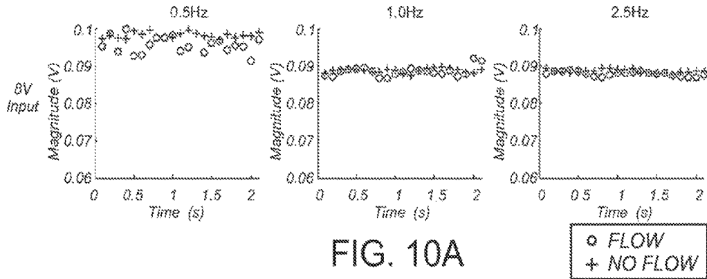
Elongate Member #1 Resistive Member #4: Magnitude Plot
